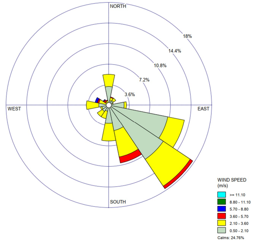
Figure A8 Wind Speed and Direction (March 2025)
