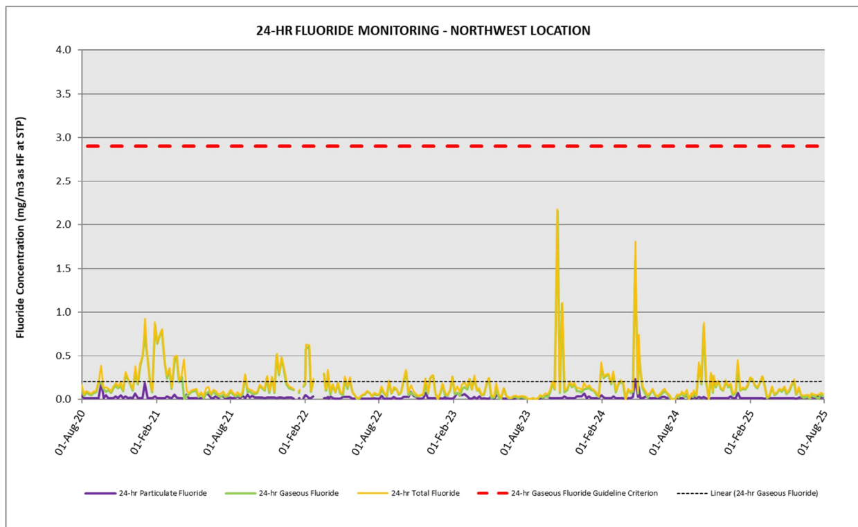
Figure 15 24-hour fluoride monitoring results – Northwest location (2020 – 2025)
