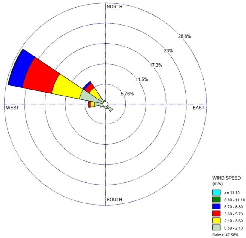
Figure A1 Wind Speed and Direction (August 2024)
