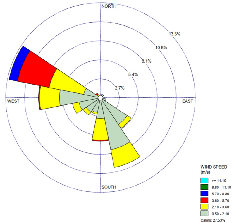
Figure A10 Wind Speed and Direction (May 2025)
