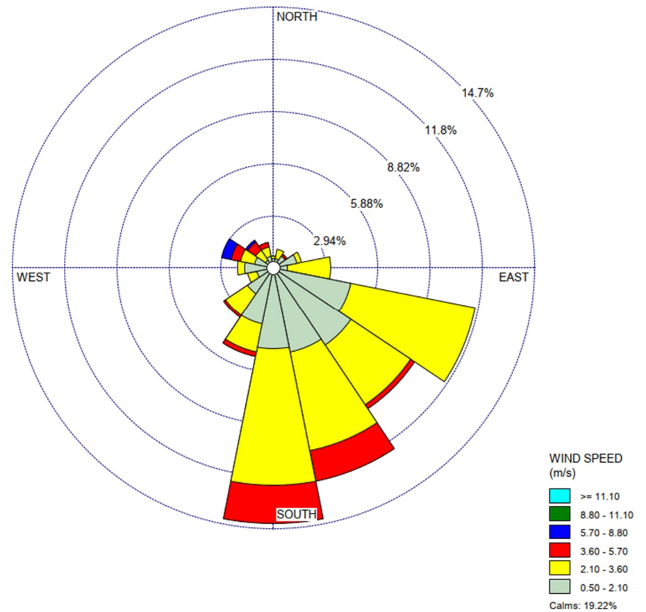
Figure A6 Wind Speed and Direction (January 2025)
