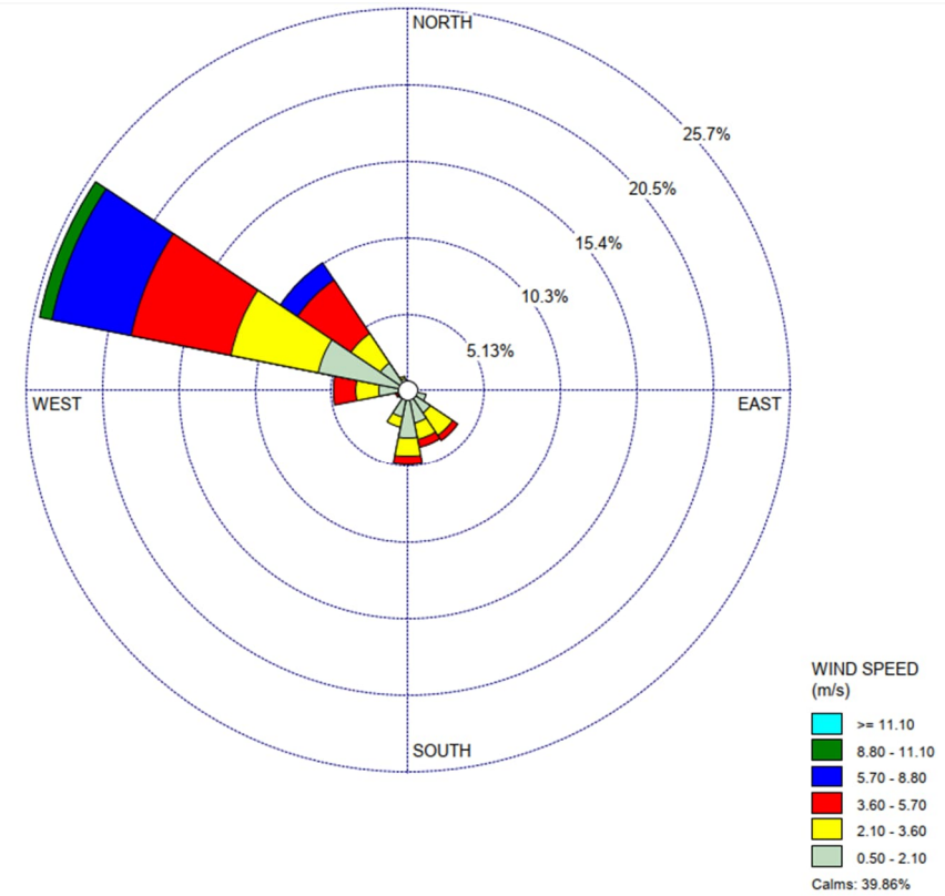
Figure A2 Wind Speed and Direction (September 2024)
