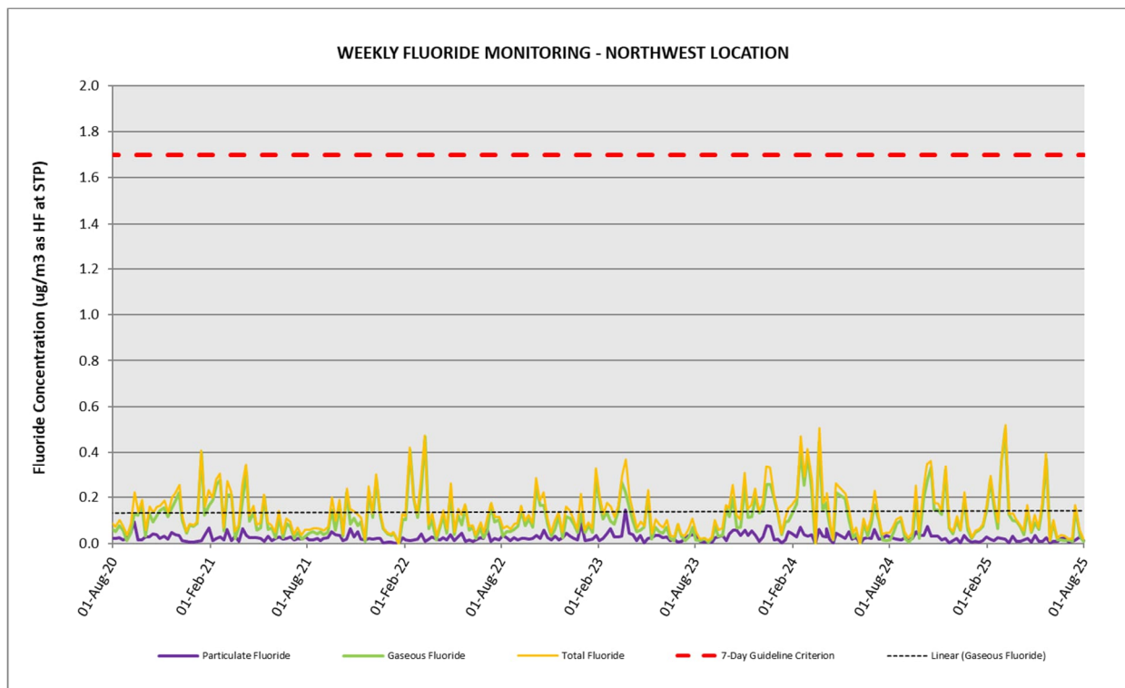
Figure 17 Weekly fluoride monitoring results – Northwest location (2020 – 2025)
