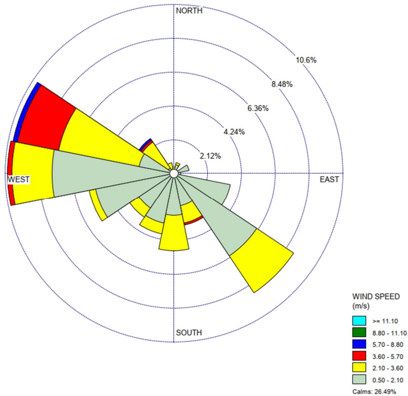
Figure A9 Wind Speed and Direction (April 2025)
