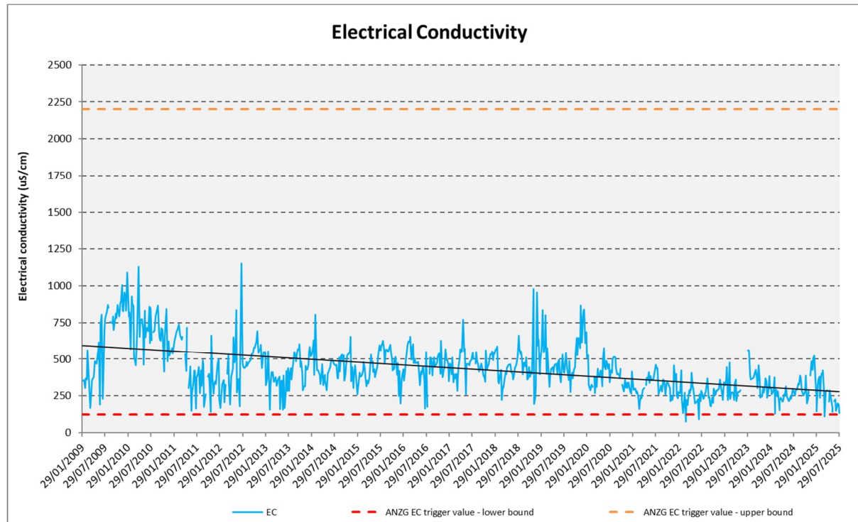
Figure 28 Stormwater quality, Pond 4 – EC (2009-2025)
