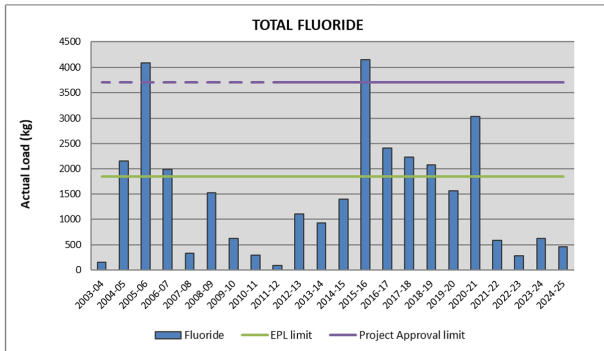
Figure 21 Fluoride annual load (2004 – 2025)
