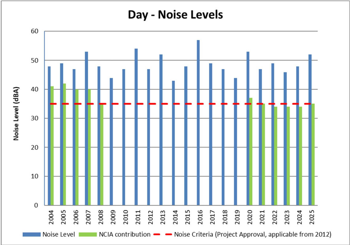
Figure 24 Day noise levels, Kenvil Close, 2004 – 2025
