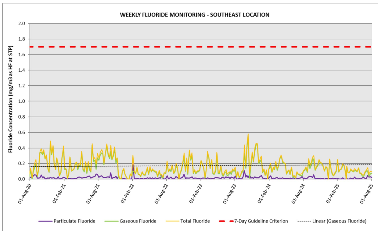
Figure 18 Weekly fluoride monitoring results – Southeast location (2020 – 2025)
