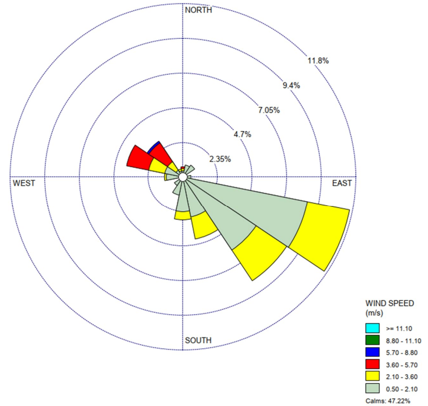
Figure A4 Wind Speed and Direction (November 2024)
