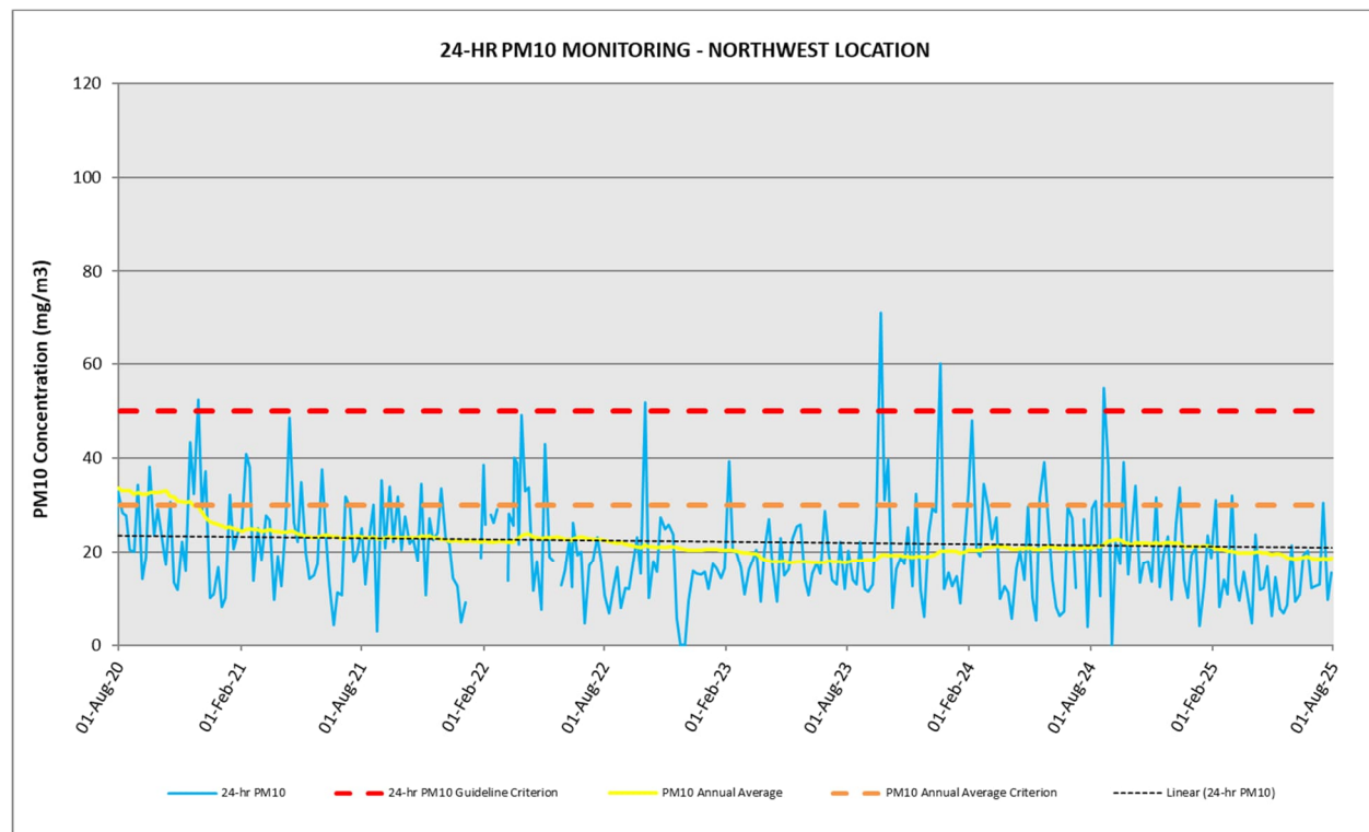
Figure 13 24-hour PM 10 monitoring results – Northwest location (2020 – 2025)
