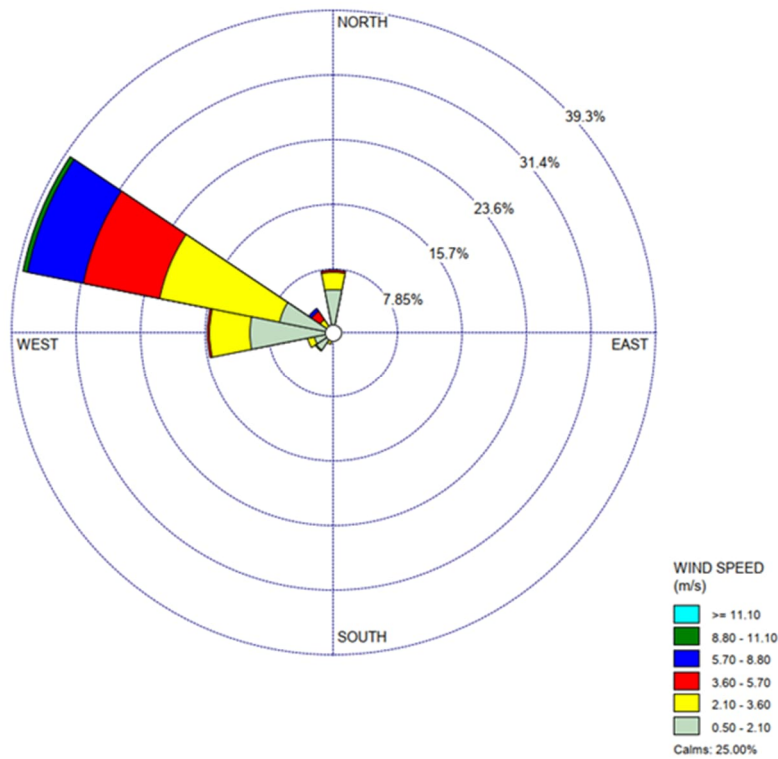
Figure A11 Wind Speed and Direction (June 2025)
