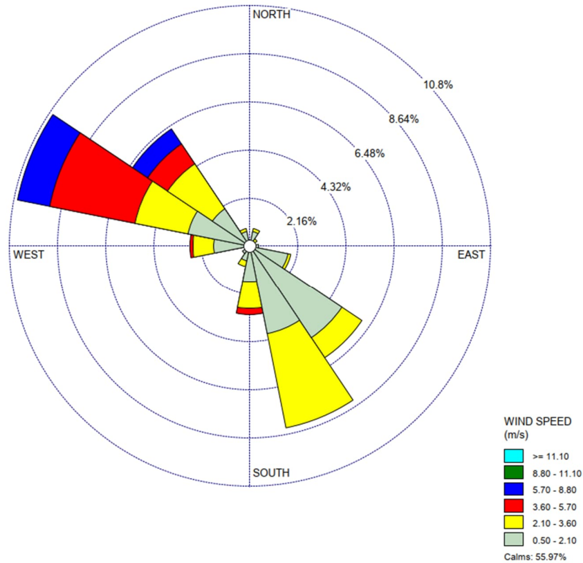
Figure A3 Wind Speed and Direction (October 2024)
