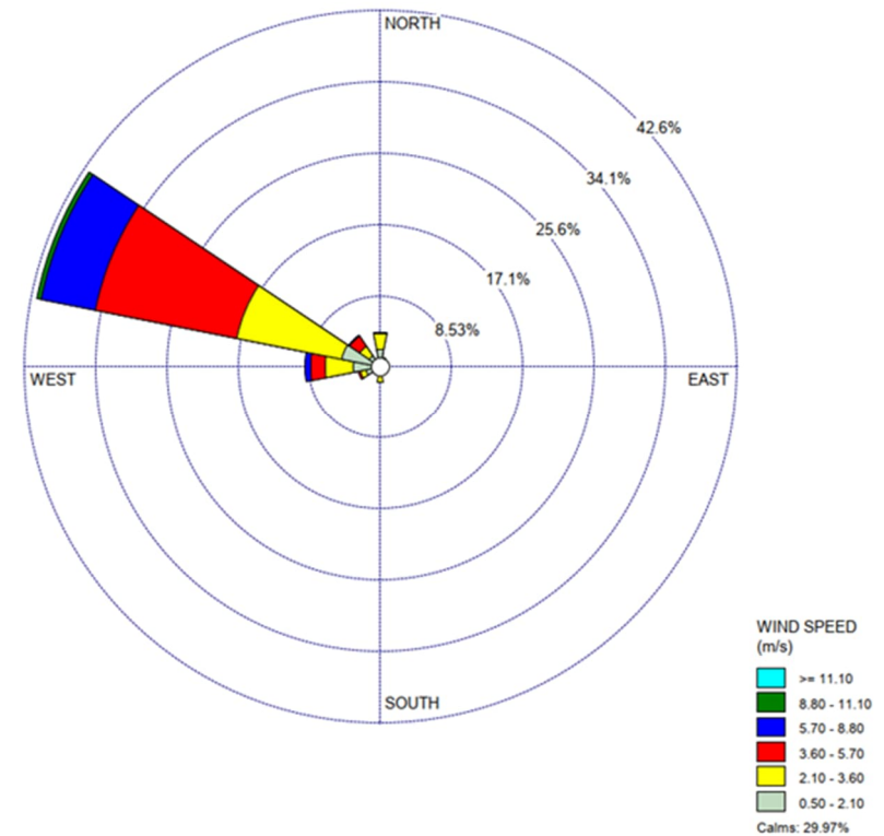
Figure A12 Wind Speed and Direction (July 2025)
