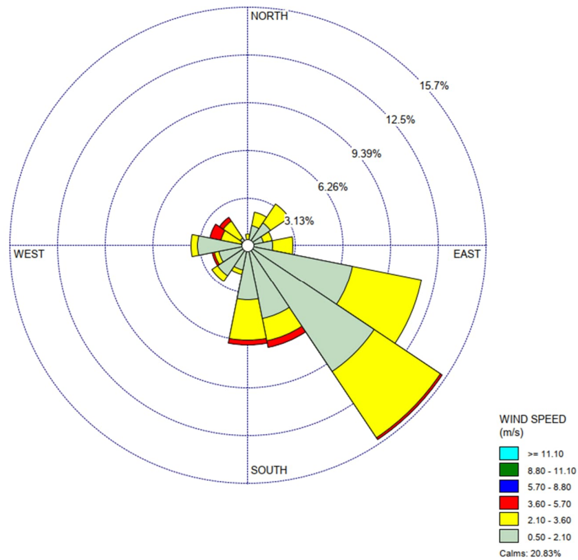
Figure A7 Wind Speed and Direction (February 2025)
