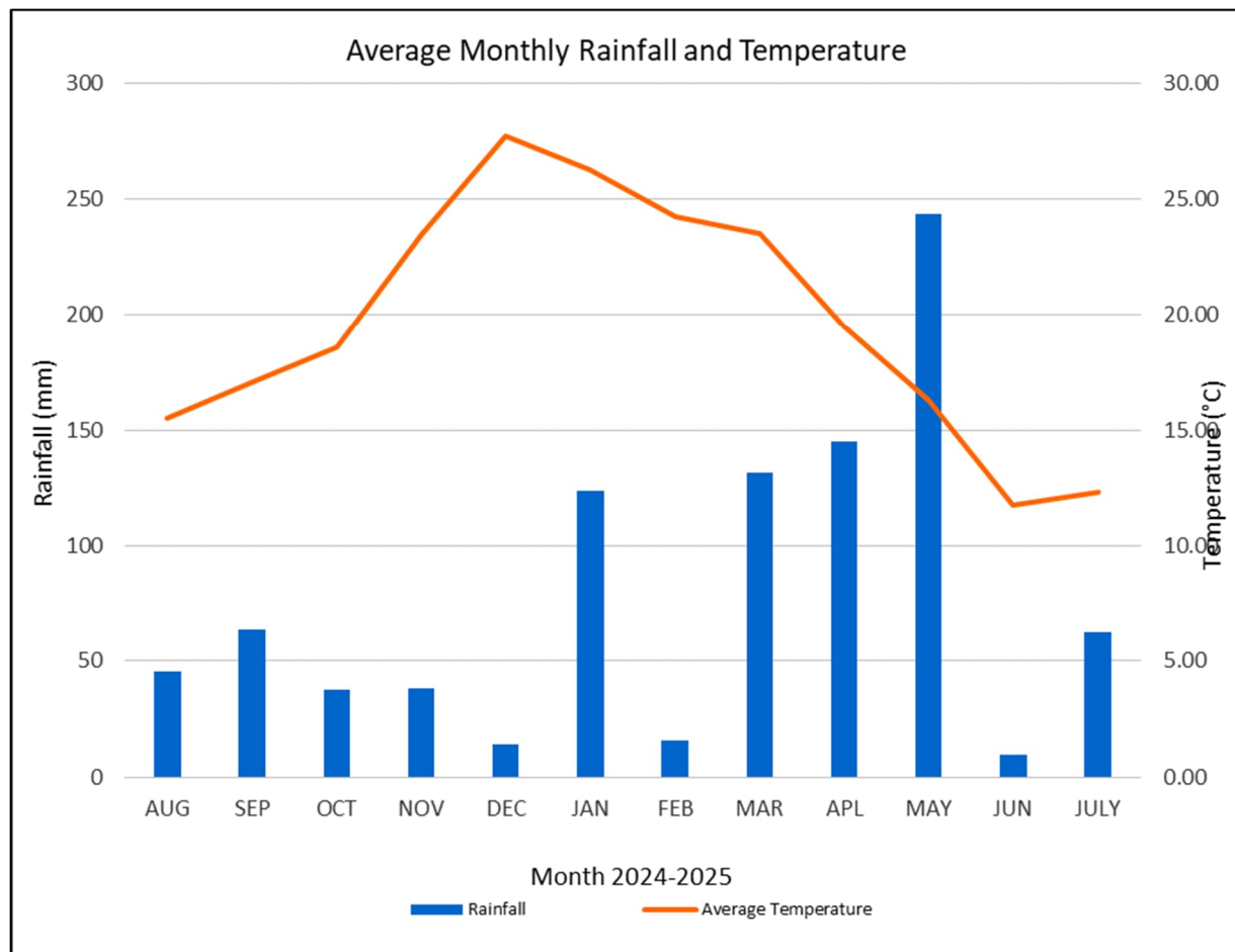
Figure 9 Average monthly rainfall and temperature range (1 August 2024 – 31 July 2025)
