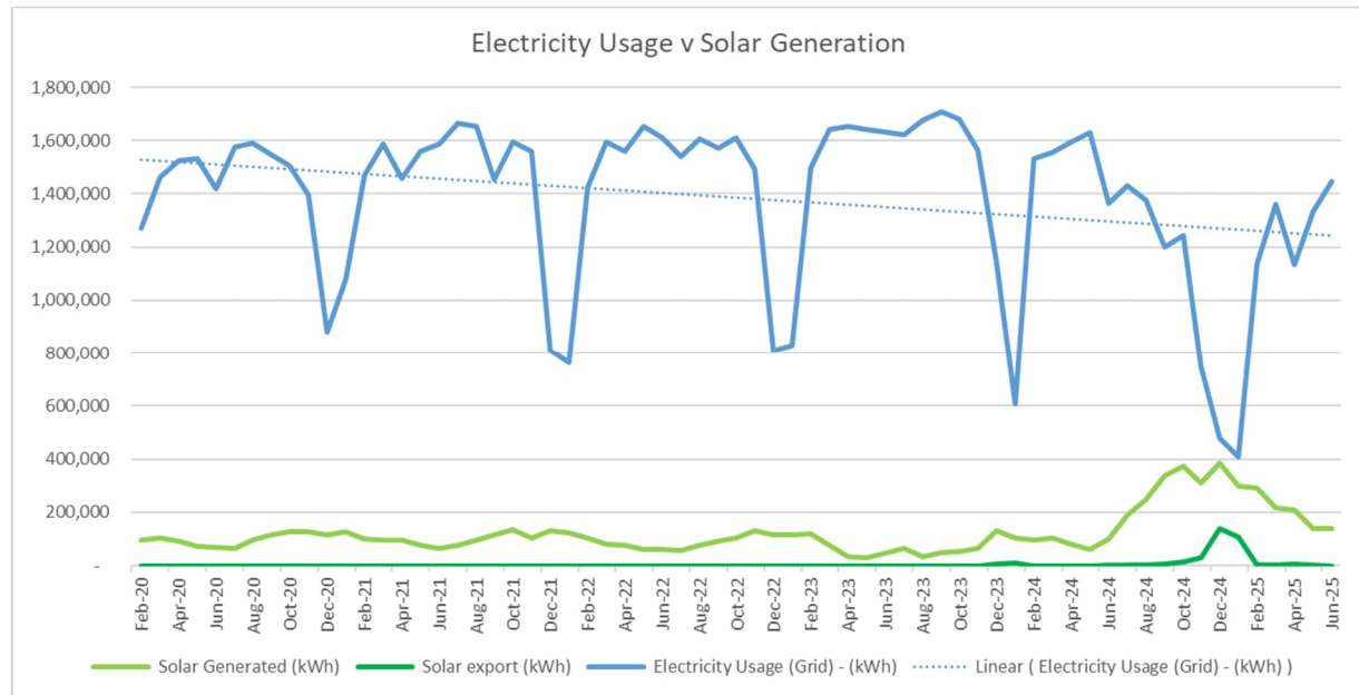
Figure 30 Electricity Usage and Solar Generation
