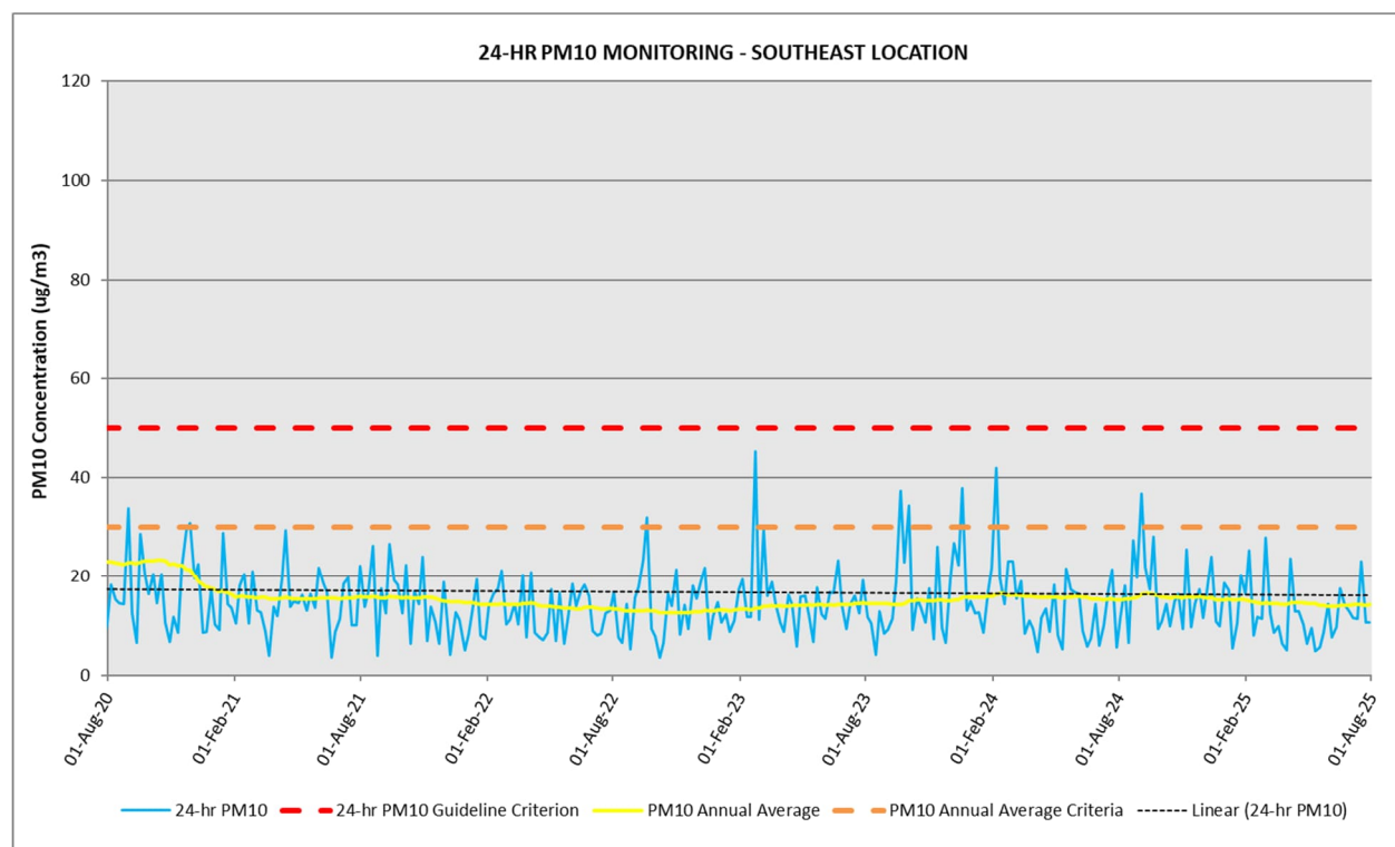
Figure 14 24-hour PM 10 monitoring results – Southeast location (2020 – 2025)
