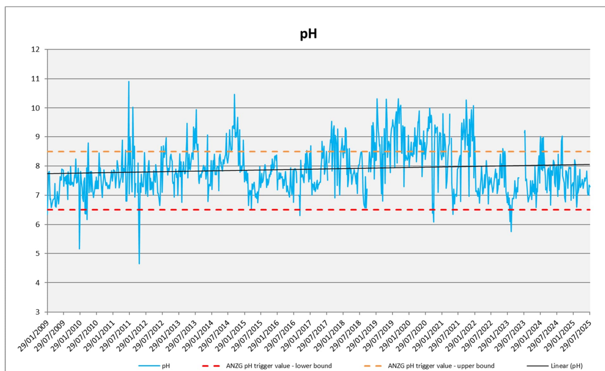
Figure 27 Stormwater quality, Pond 4 pH (2009-2025)
