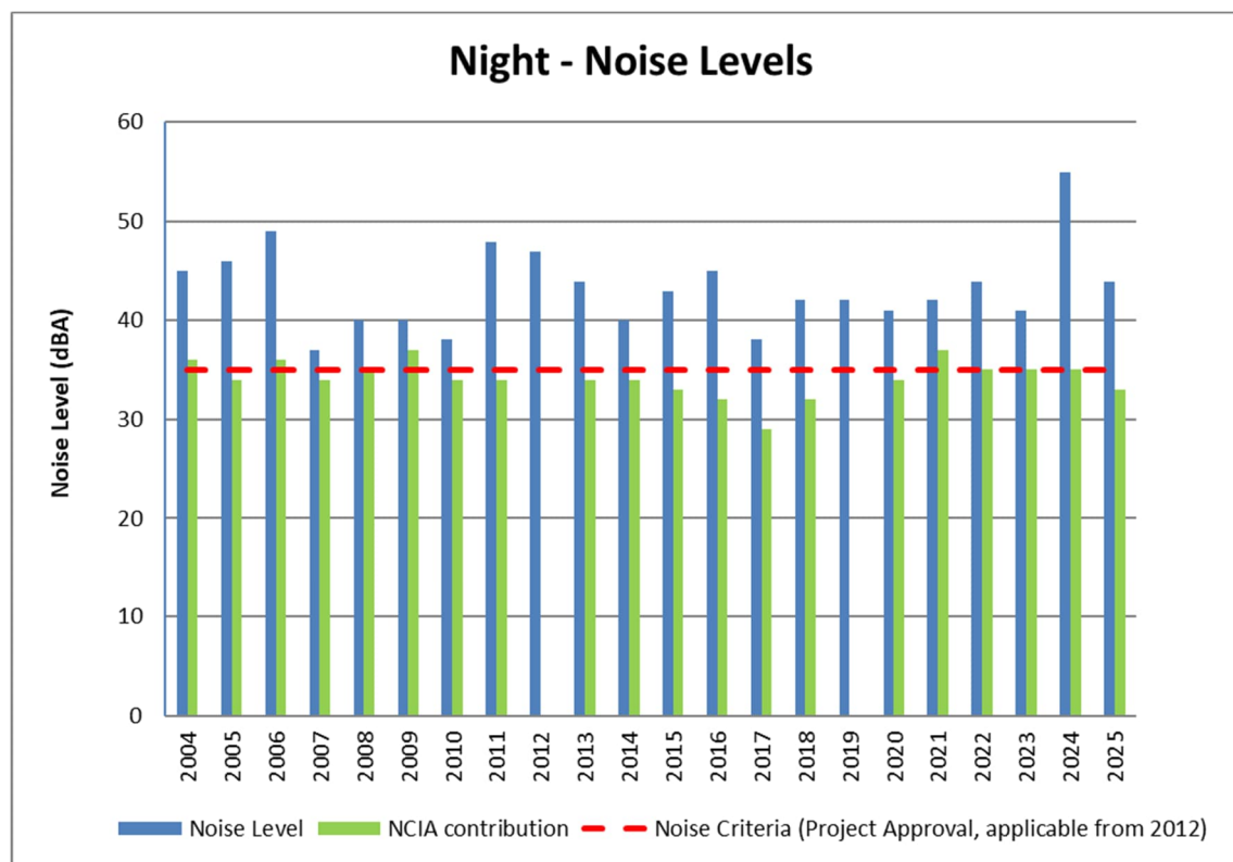
Figure 26 Night noise levels, Kenvil Close, 2004 – 2025
