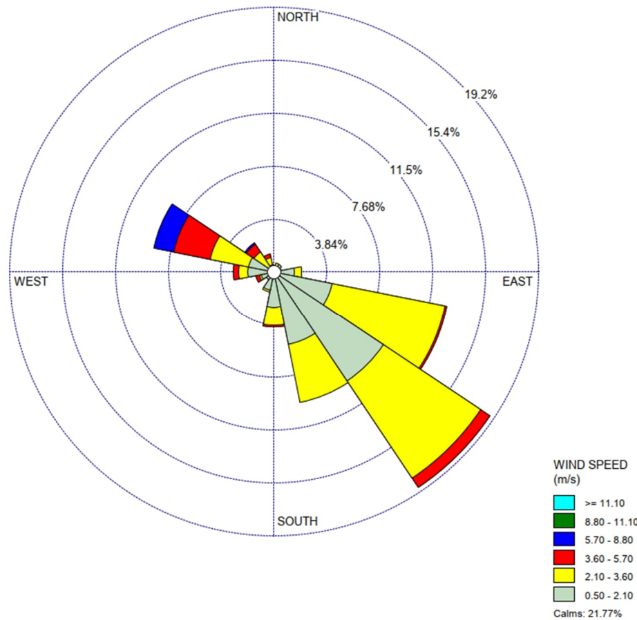
Figure A5 Wind Speed and Direction (December 2024)
