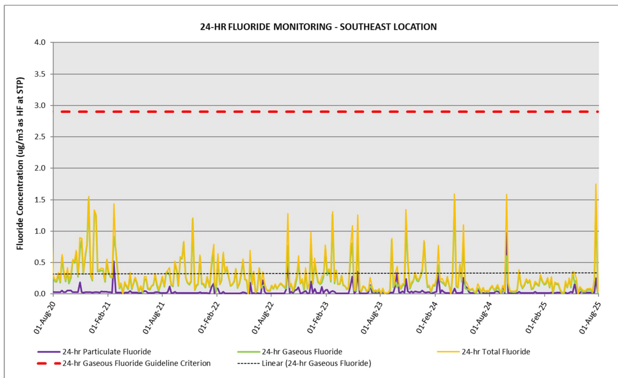
Figure 16 24-hour fluoride monitoring results – Southeast location (2020 – 2025)
